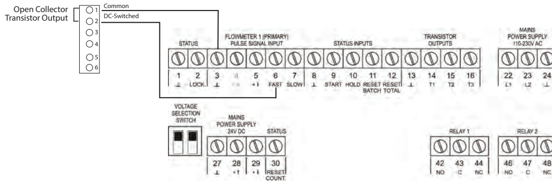
Figure 20: Wiring to a PC-200 controller
