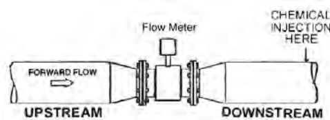
Figure 9: Chemical injection point upstream of meter
