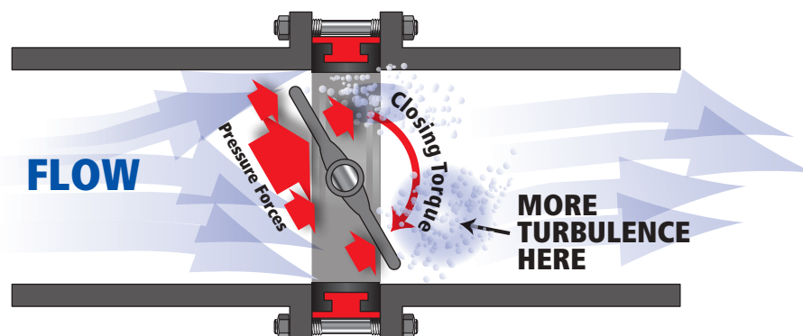
Figure 1 - Pressure Distribution
